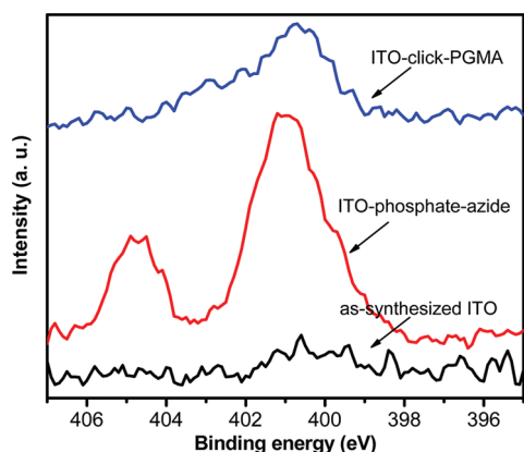
Figure 5. XPS scan of N1s of as-synthesized ITO, phosphate–azide treated ITO, and PGMA grafted ITO nanoparticles.
