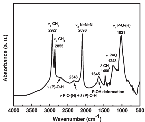
Figure 2. FTIR spectrum of 11-azidoundecyl dihydrogen phosphate.
