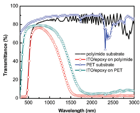
Figure 10. UV–vis–NIR transmittance spectra of 35 wt % ITO-epoxy coating (with thickness of 5 \mu\text{m} ) on plastic substrates.
