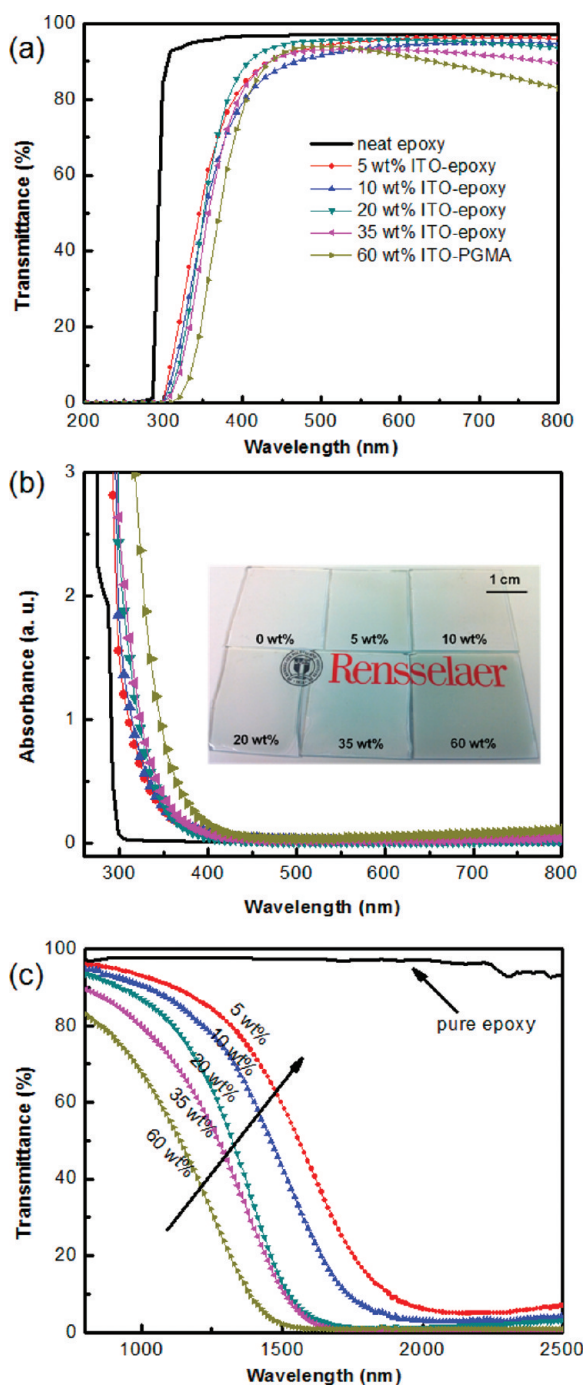
Figure 9. UV–vis spectra of ITO/epoxy nanocomposites with different ITO contents (a) transmittance and (b) absorbance (the inset pictures are digital photographs of 20 \mu\text{m} thick ITO/epoxy coating on glass substrate with thickness); (c) near IR transmittance spectra of ITO/epoxy nanocomposites.
