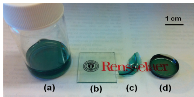
Figure 7. Photographs (a) ITO/PGMA dispersion in chloroform, (b) ITO/PGMA coating on glass slides, (c) 100 \mu\text{m} thick ITO/PGMA composites after removal of solvent (60 wt % ITO loading), (d) ITO/epoxy composites (20 wt % ITO loading, 3 mm thick).
