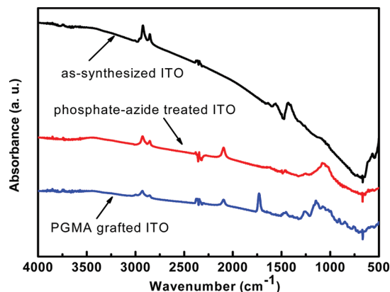
Figure 4. FTIR spectra of as-synthesized ITO, phosphate-azide treated ITO, and PGMA grafted ITO nanoparticles.
