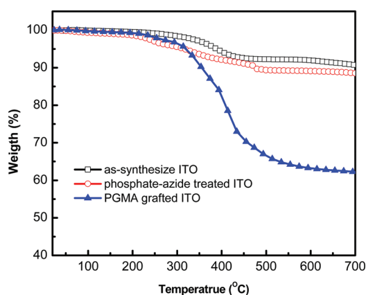
Figure 6. TGA curves of as-synthesized ITO nanoparticles, phosphate–azide treated ITO nanoparticles, and PGMA grafted ITO particles.
