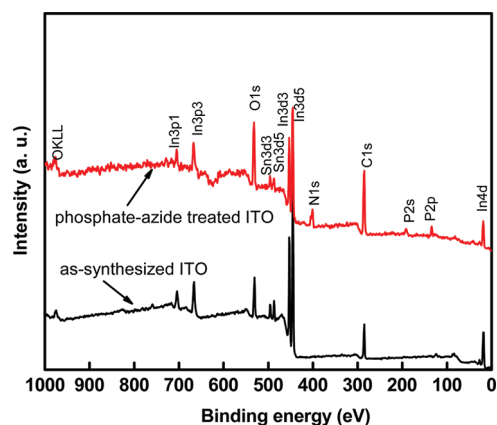
Figure 3. XPS survey of synthesized ITO and ITO particles treated with phosphate-azide.
