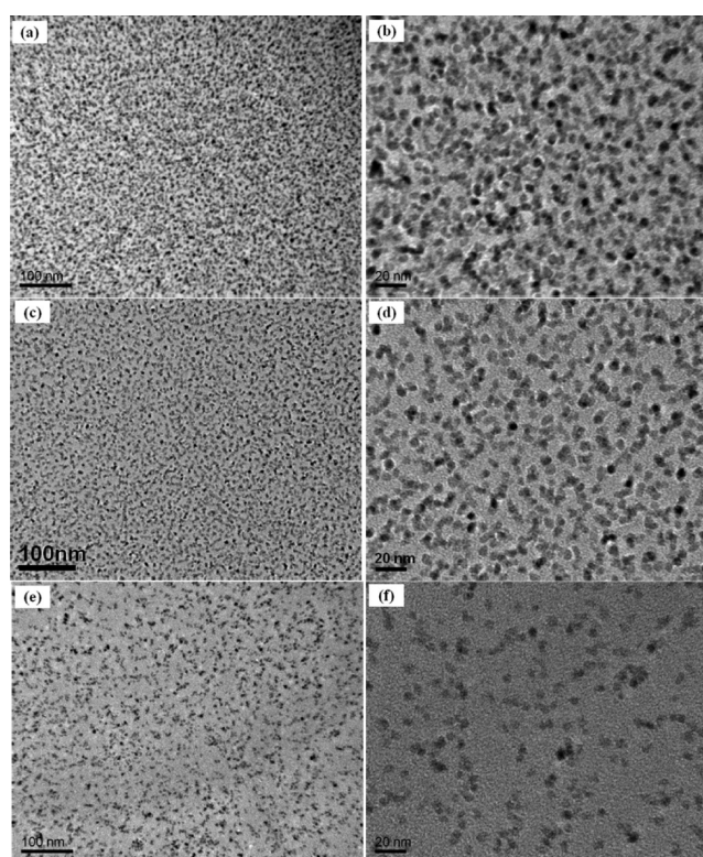
Figure 8. TEM image of ITO/epoxy nanocomposites with different ITO concentrations at low and high magnifications: (a, b) 35 wt %; (c, d) 20 wt %; (e, f) 10 wt %.
