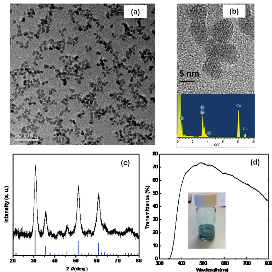
Figure 1. (a) TEM image of synthesized ITO nanoparticles, (b) HRTEM image with TEM-EDS analysis, (c) XRD diffraction pattern, (d) transmittance spectrum of ITO dispersion in hexane (10 mg/mL) measured through a quartz cuvette and inset photograph of green ITO dispersion.
